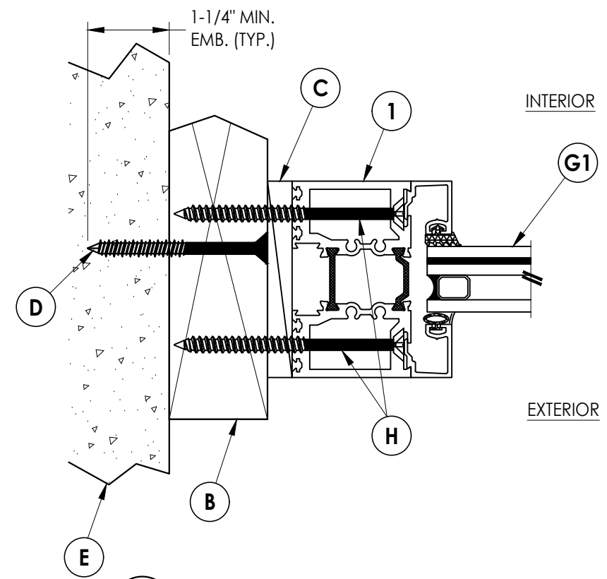
3 HORIZONTAL CROSS SECTION
